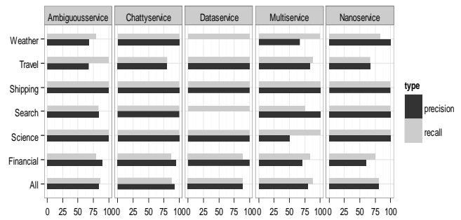
Figure 5. Detection results for each antipattern type.
