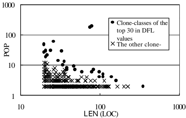
Figure 5. Population and length of clone-classes in JDK
