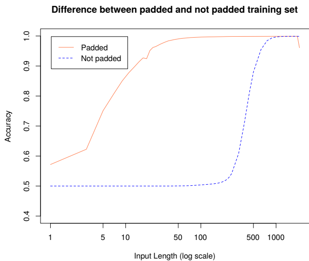
Fig. 11. Accuracy of the LSTM model if it has been trained with padded values or not
